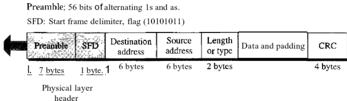
Figure 4 802.3 MAC frame
