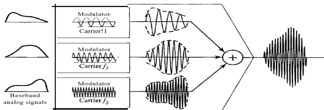
Figure 2 FDM process
